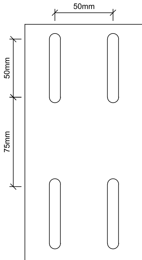
TS1 9.5mm Wide Slots Open Area: 8.7%
